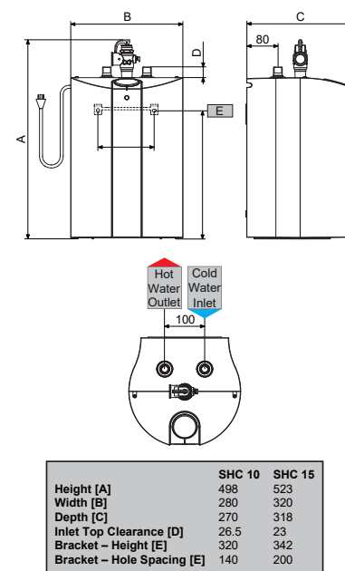
SHC Dimensions
