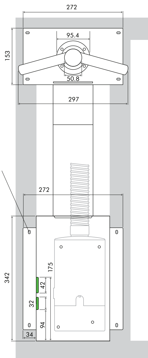
FRONT ELEVATION
