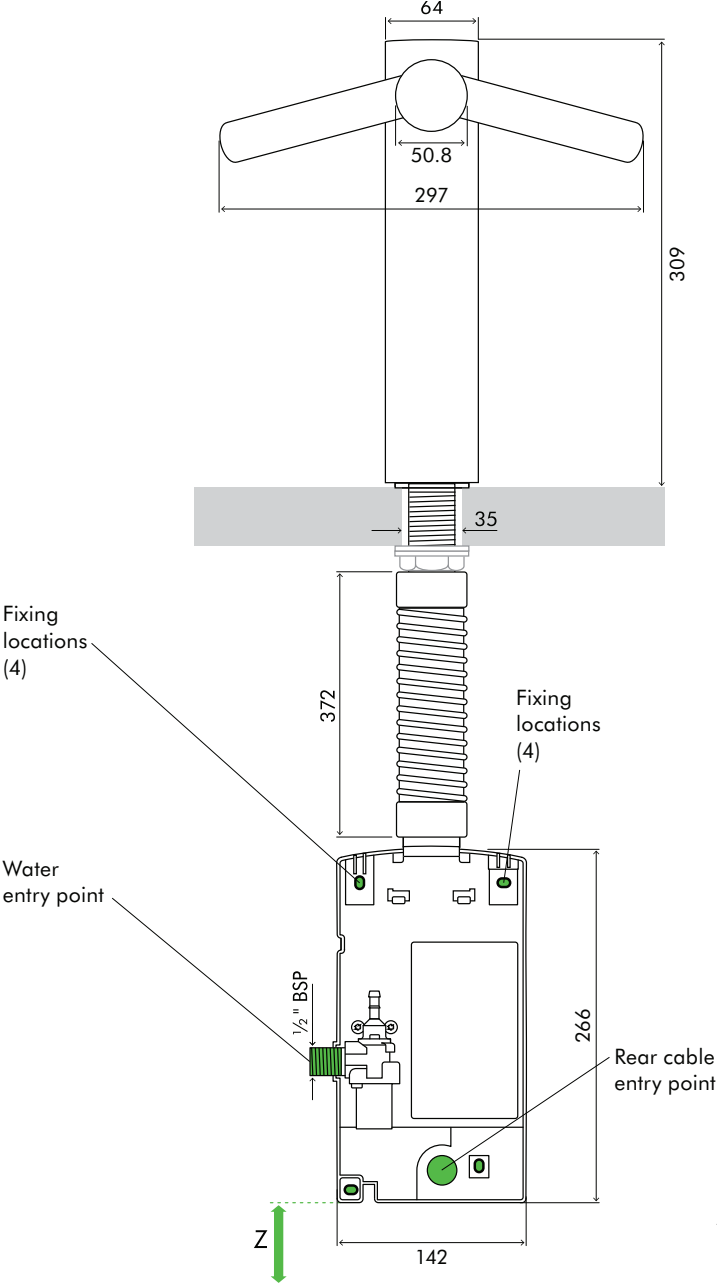
FRONT ELEVATION
